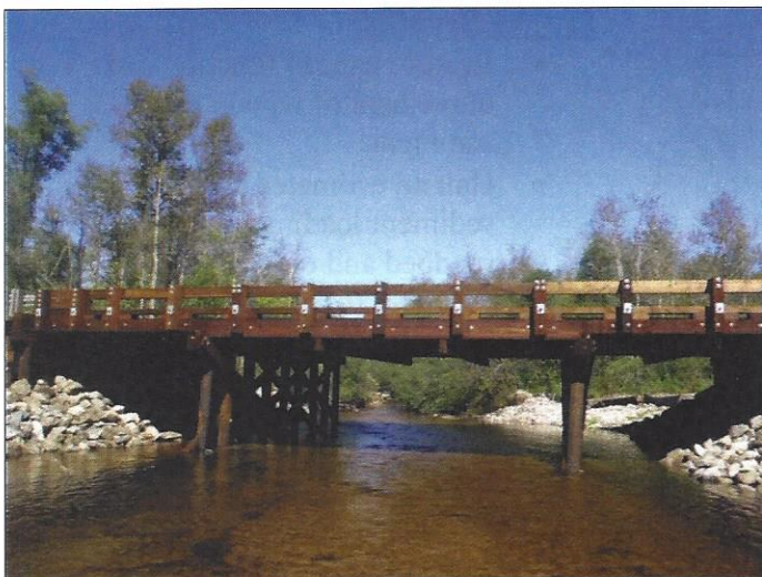
During – The timber deck and restored river channel.
