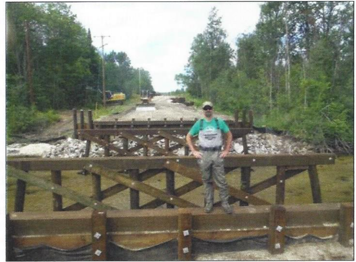
During – Timber piles and abutments were installed
